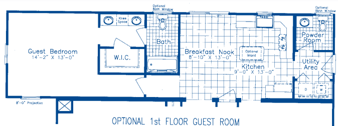
OPTIONAL 1st FLOOR GUEST ROOM
